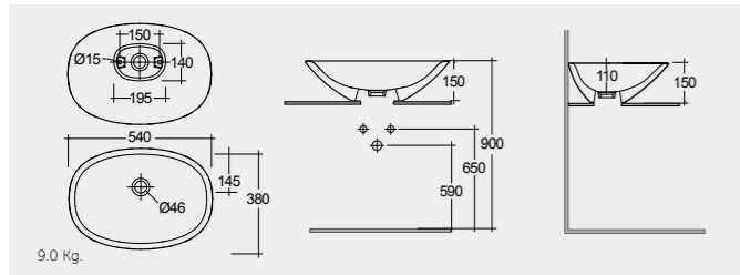
MORCT5400AWHA Oval
